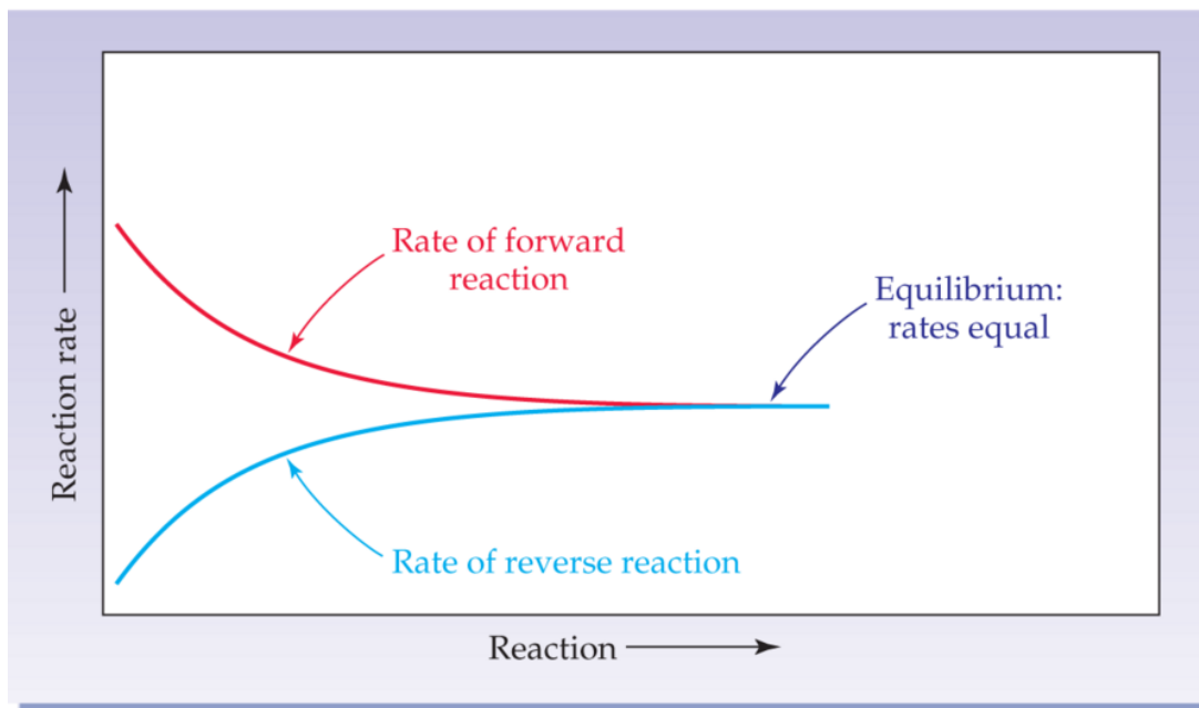
Figure 7.6 Reaction rates in an equilibrium reaction.
